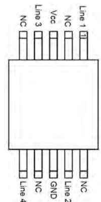
Pin Schematic
