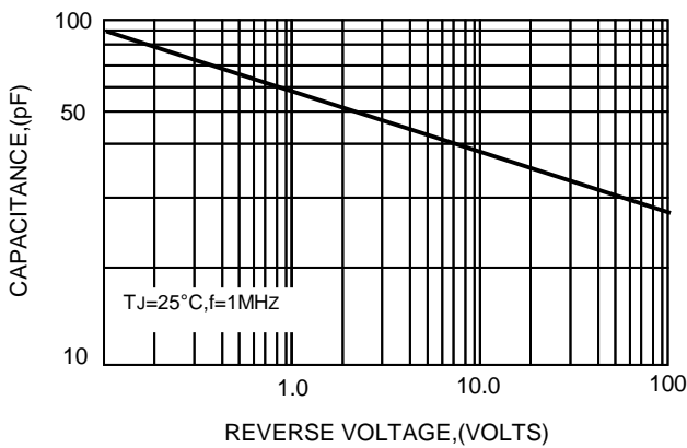
FIG.5-TYPICAL JUNCTION CAPACITANCE
