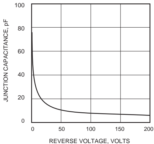
FIG.7 - TYPICAL JUNCTION CAPACITANCE
