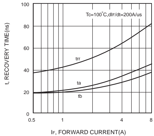
FIG.6 - trr, ta AND tb CURVES vs FORWARD CURRENT
