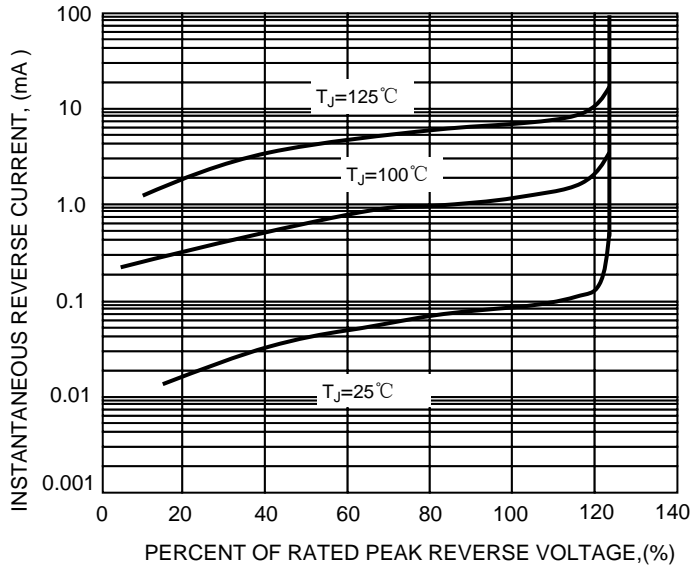
FIG.5-TYPICAL REVERSE CHARACTERISTICS
