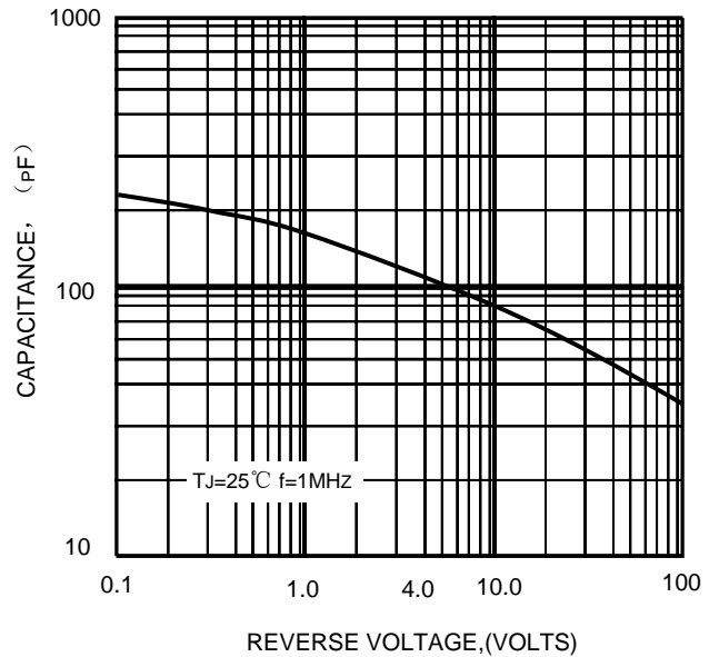
FIG.4-TYPICAL JUNCTION CAPACITANCE
